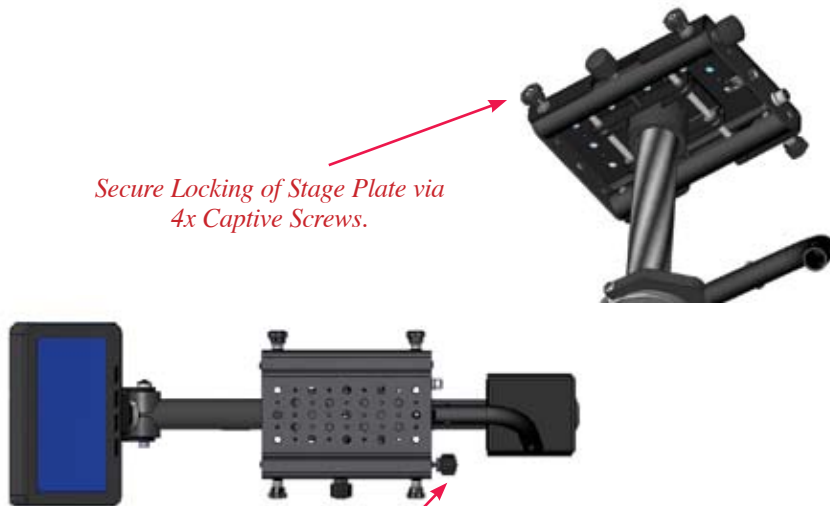
Stage Plate has X-Y Vernier Adjustment.
