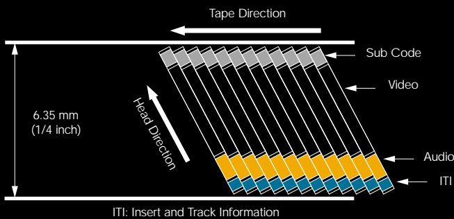
Track Pattern of the DVCAM Format
