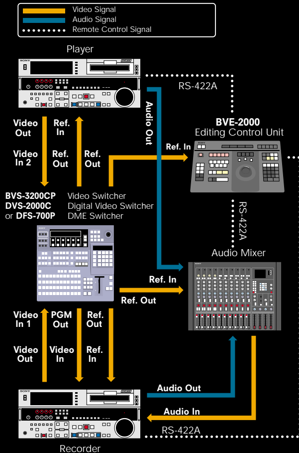
Preread Editing System
